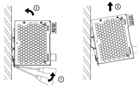
Fig. 2.2 Dismounting
