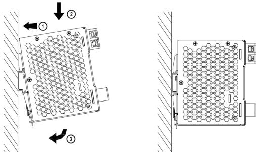
Fig. 2.1 Mounting
