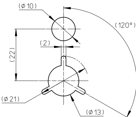
DETAIL "D"
