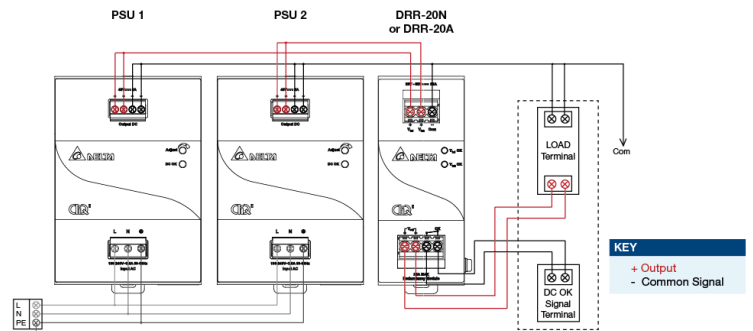
Fig. 4 Redundant Operation Connection Diagram
