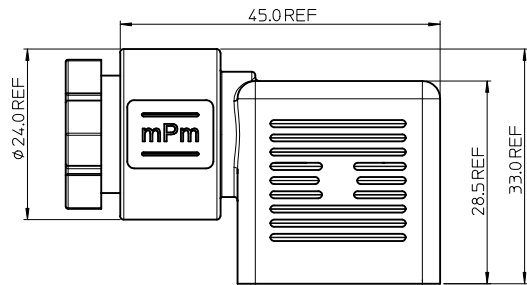
COVER DIMENSIONS FOR M20x1.5 AND 1/2" NPTF THREADED CONNECTORS
