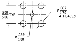
Recommended PCB Hole Configuration
